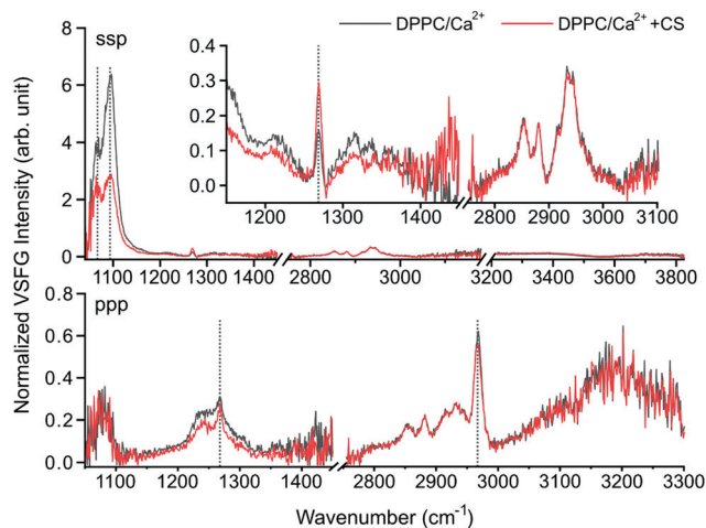
Fig. 2 The ssp (top) and ppp (bottom) polarization VSFG spectra of a \sim 30 mN m^{-1} DPPC monolayer over a 2.8 mM Ca^{2+} solution as subphase with (red trace) and without (black trace) CS. The inset shows the magnified sections of 1150–1450 cm^{-1} and 2750–3180 cm^{-1} .
