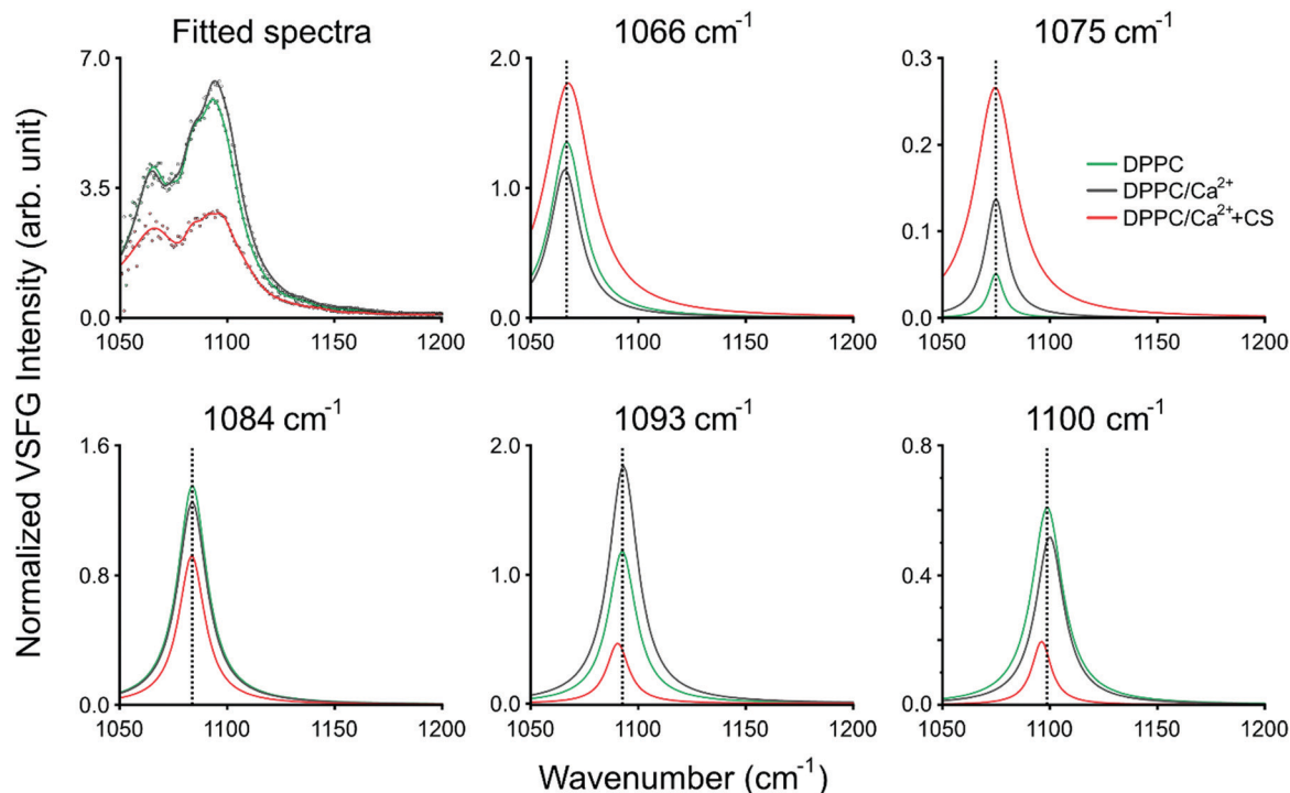
Fig. 3 Results of the Lorentzian fitting of the VSFG spectra. The sum of all fitted peaks is shown on the top left. The different panels present the 1066 cm^{-1} (top middle), 1075 cm^{-1} (top right), 1084 cm^{-1} (bottom left), 1093 cm^{-1} (bottom middle), and 1100 cm^{-1} (bottom right) peaks fitted to the spectrum of DPPC on a 2.8 mM Ca^{2+} subphase without (black traces) and with (red trace) CS. As a control, the panels also contain the corresponding fitted spectrum and peaks of DPPC on pure H_2O (green traces). The fitting parameters are listed in Table S1 in the ESI.†
